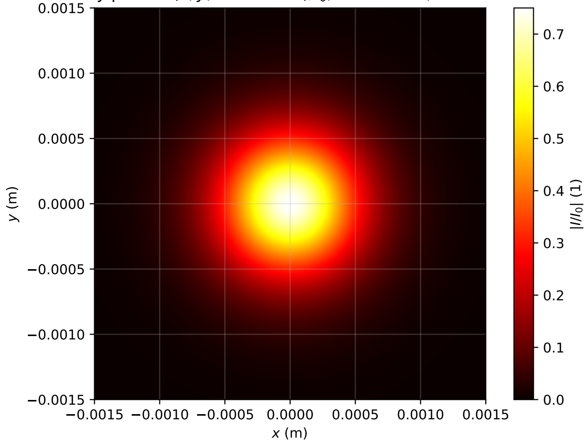
Intensity profile I(x, y, z = 2.707m)/I_0 , Pin=0.6Pcr, artificial time
